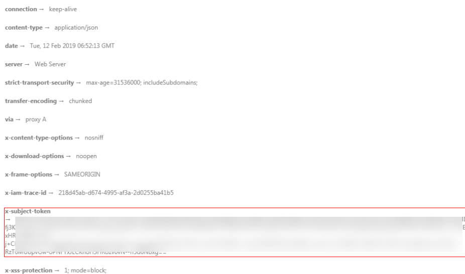
Figure 3-5 Header fields of the response to the request for obtaining a user token
